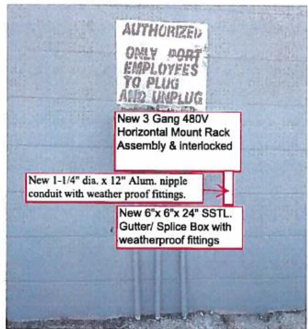
New configuration of 3 Gang Reefer Outlets 480V/ 3PH/32Amps
