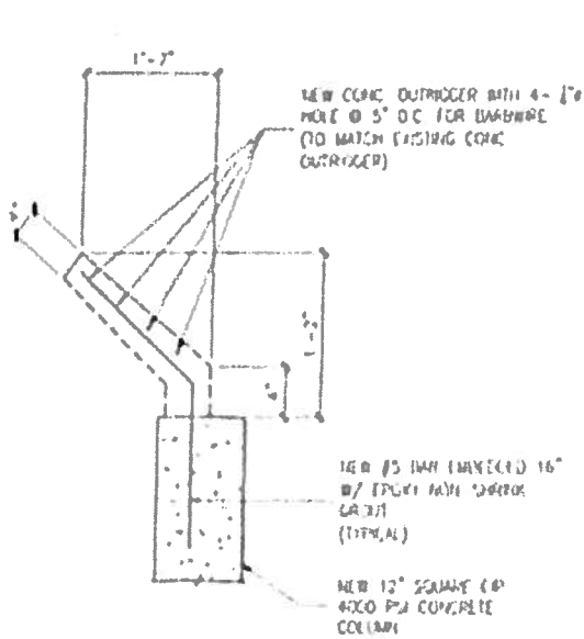
7 TYPICAL COLUMN CORNER REPAIR C-2 SCALE 1" = 1'-0"
