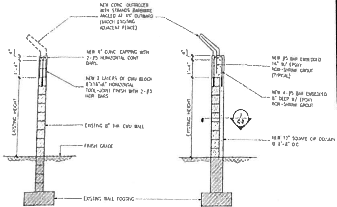
4 CMU WALL SECTION C-2 SCALE 1/2" = 1'-0"
